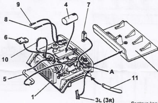
Sestava kapoty motoru Bonet assembly
