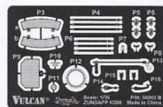
Photo-Etched Parts
